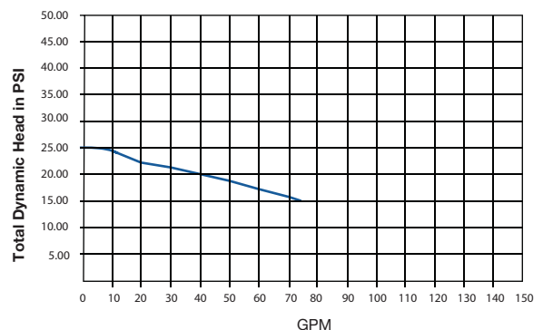
Performance Curve Marathon Motor 9.0 Amp PSI/GPM
