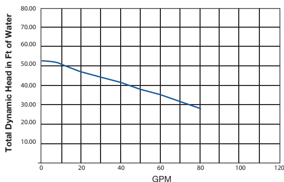
Performance Curve Marathon Motor 9.0 Amp Feet of Water/GPM
